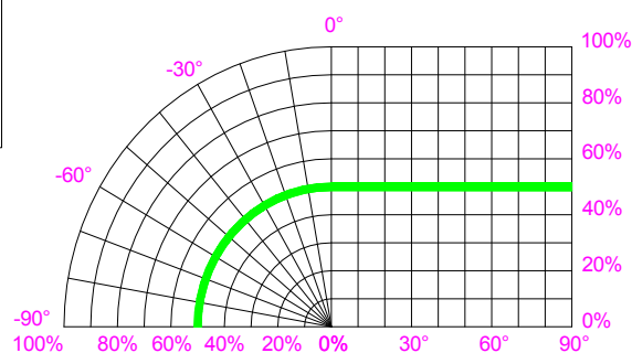
Directive Characteristics
